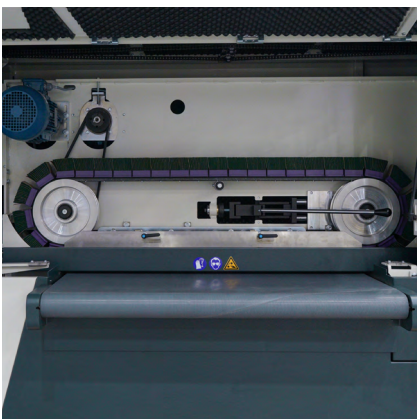
__ 2 counter-rotating cross-belts
